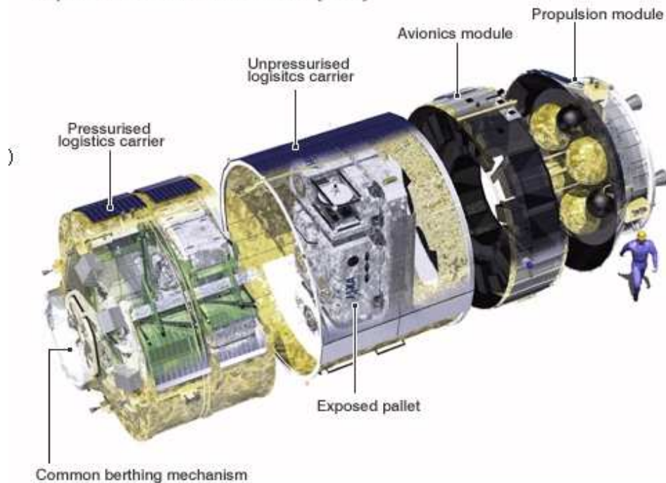
Japan's H-II Transfer Vehicle (HTV)
